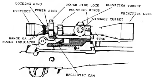
Figure 2-14. ART I scope.
